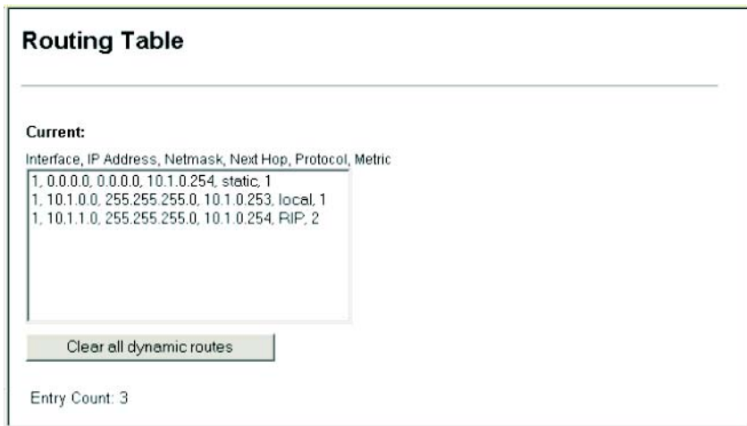
Figure 3-129 IP Routing Table
