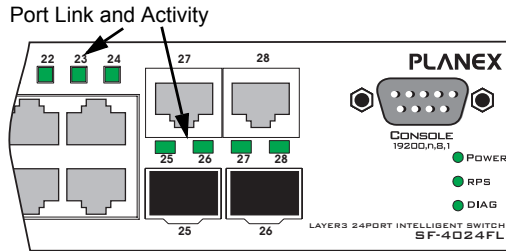
Figure 1-2 Port LEDs
