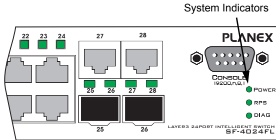
Figure 1-3 System LEDs
