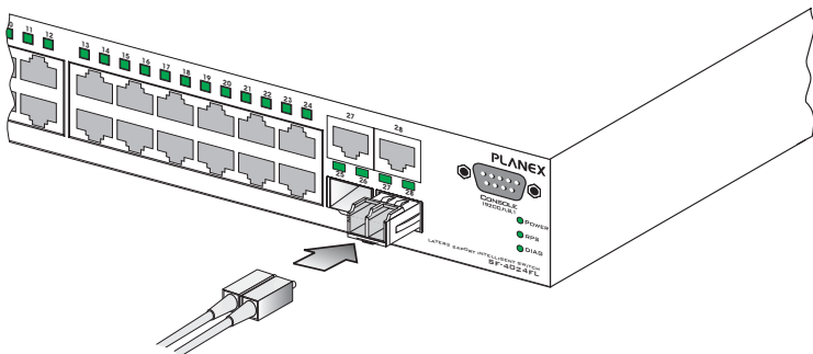
Figure 4-3 Making LC Port Connections
