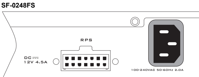
Figure 3-7 Power Receptacles
