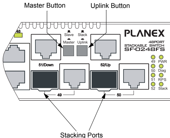
Figure 1-2 Stacking Ports
