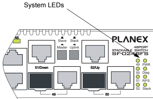
Figure 1-4 System LEDs
