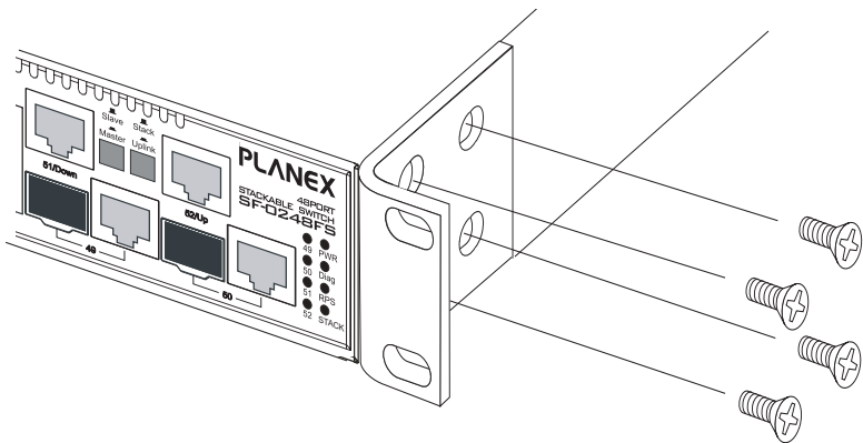
Figure 3-2 Attaching the Brackets
