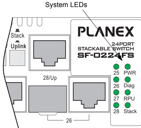
Figure 1-4 System LEDs
