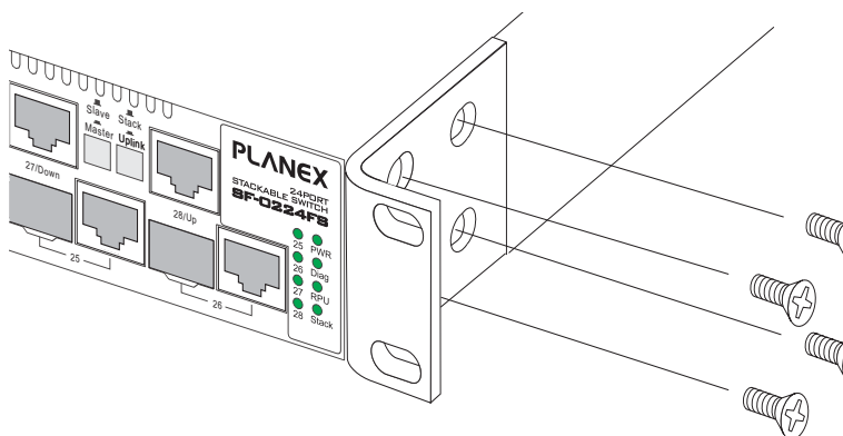
Figure 3-2 Attaching the Brackets
