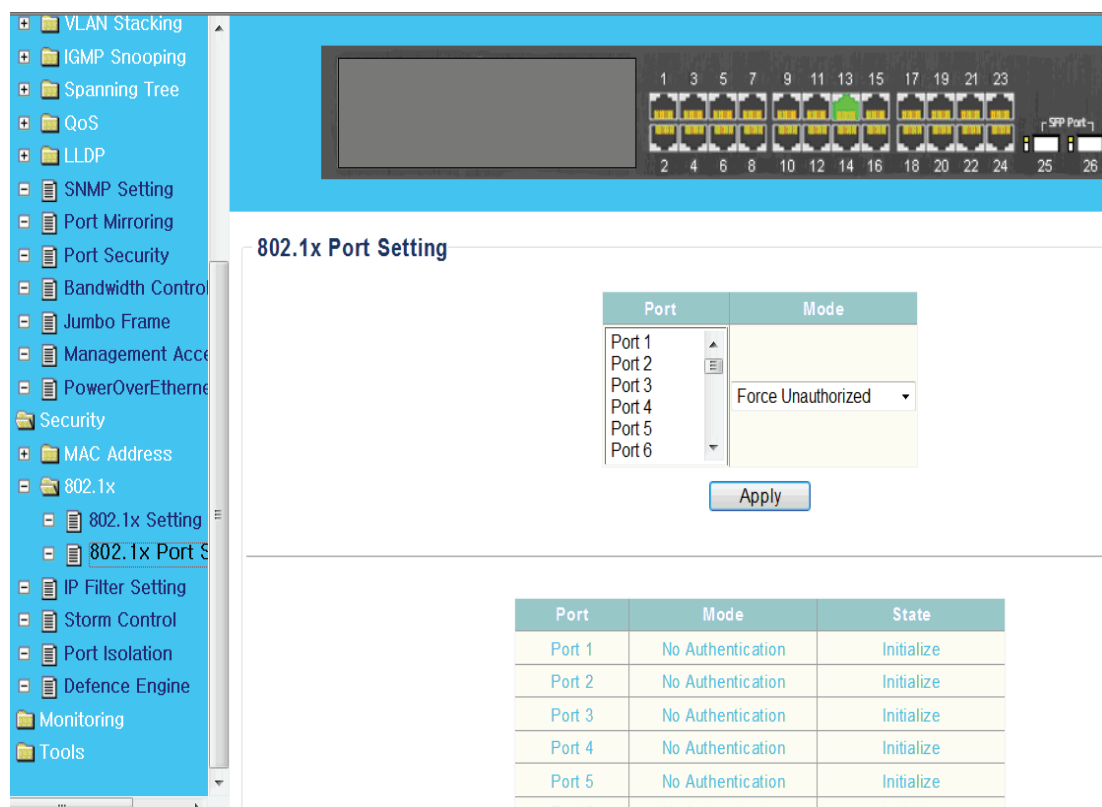
Figure 37: 802.1x Port Setting
