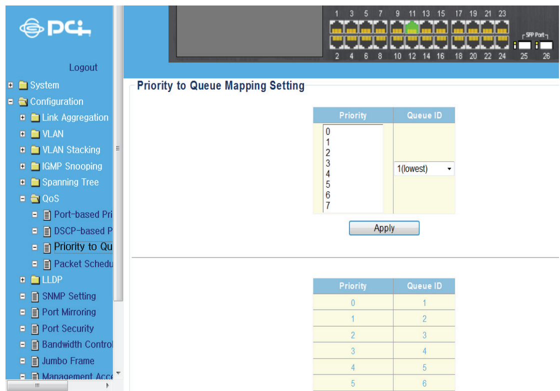
Figure 22: Priority to Queue Mapping Setting
