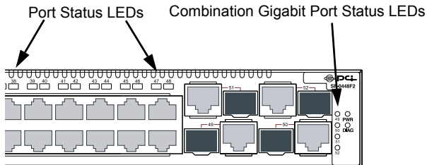
Figure 1-4. SF-0448F2 Port Status LEDs
