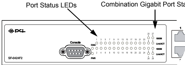
Figure 1-3. SF-0424F2 Port Status LEDs
