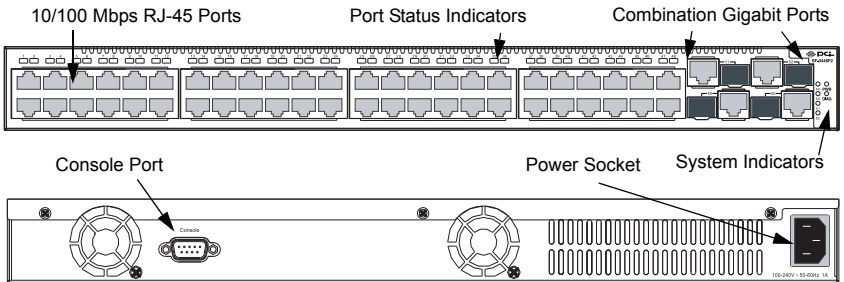
Figure 1-2. SF-0448F2 Front and Rear Panels
