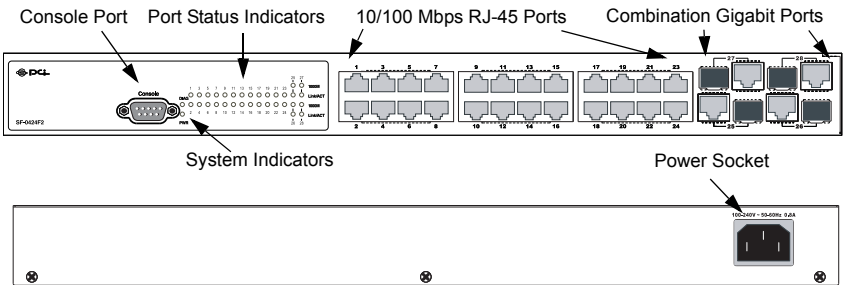
Figure 1-1. SF-0424F2 Front and Rear Panels
