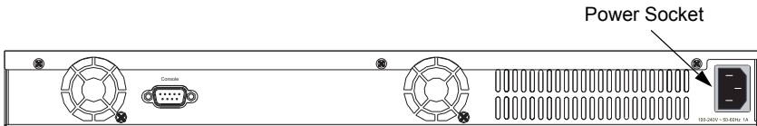
Figure 1-8. SF-0448F2 Power Supply Sockets
