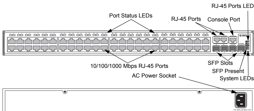
Figure 1-2. SF-0446G Front and Rear Panels
