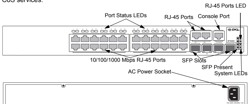
Figure 1-1. SF-0422G Front and Rear Panels
