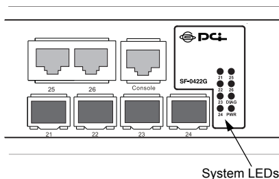
Figure 1-4. SF-0422G System Status LED
