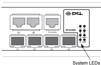
Figure 1-5. SF-0446G System Status LED
