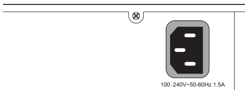
Figure 3-6. Power Sockets
