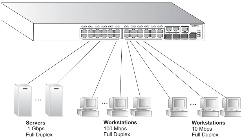
Figure 2-1. Collapsed Backbone
