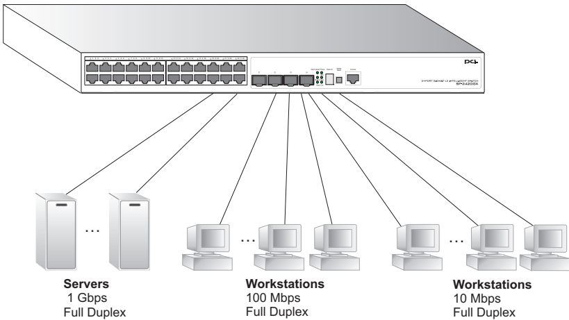
Figure 2-1 Collapsed Backbone
