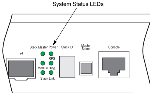
Figure 1-3 System LEDs
