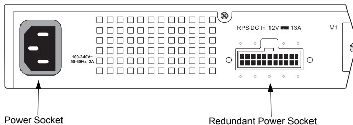
Figure 1-4 Power Supply Receptacles
